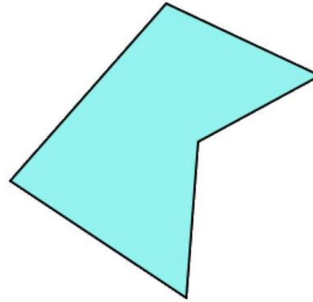
polygon
