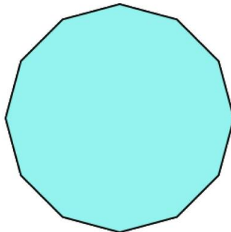
dodecagon
