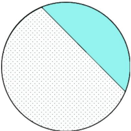
segment
