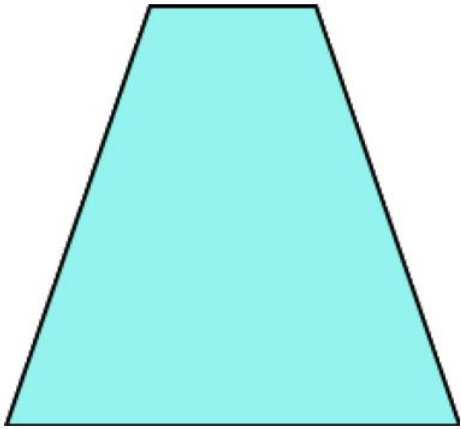
trapezoid
