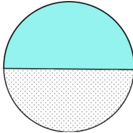
semicircle
