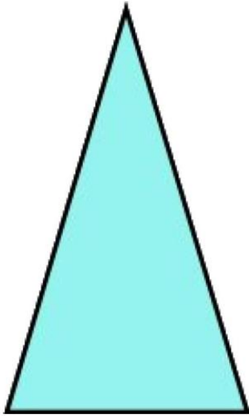
isosceles triangle
