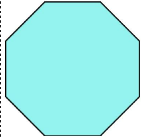
octagon
