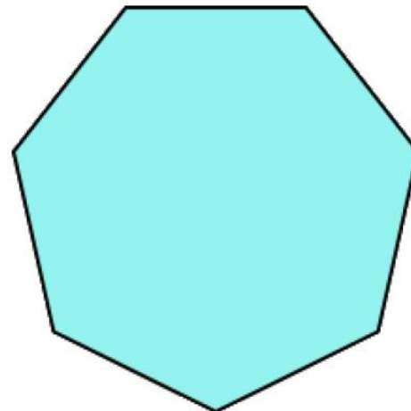
heptagon
