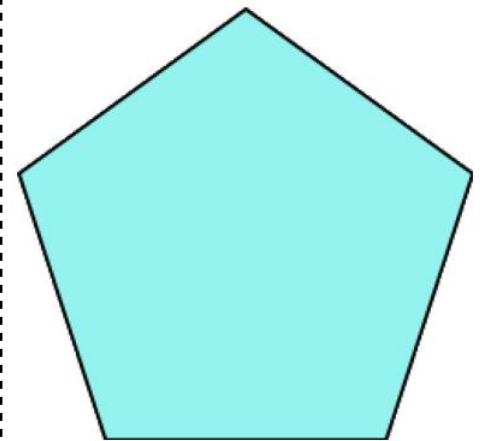
pentagon
