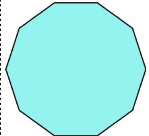
decagon
