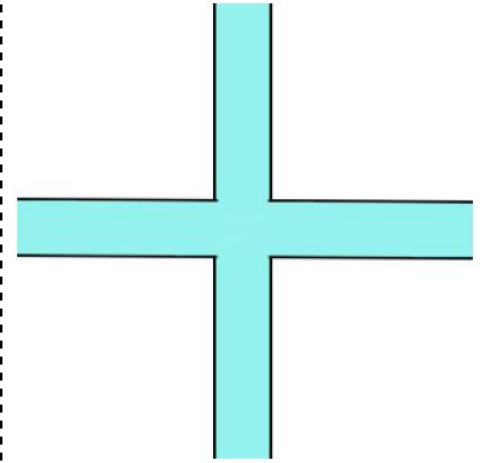
cross
