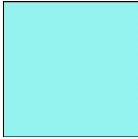
square
