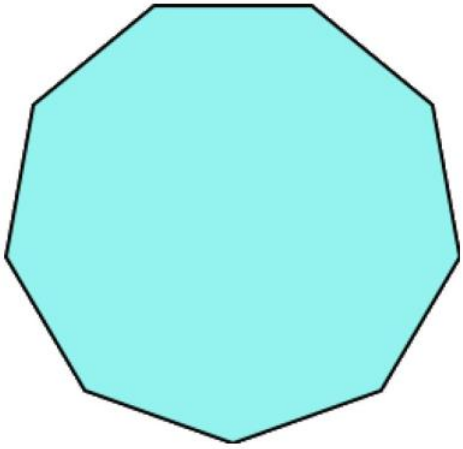
nonagon
