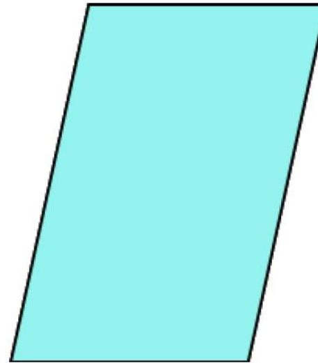
parallelogram
