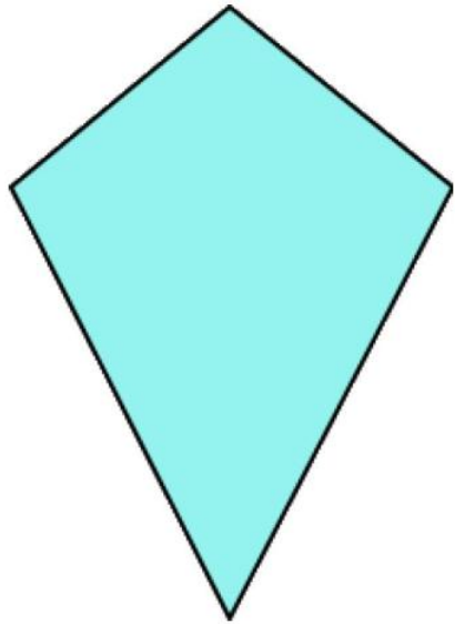
kite
