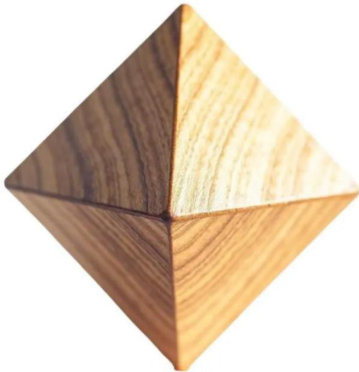
octahedron
