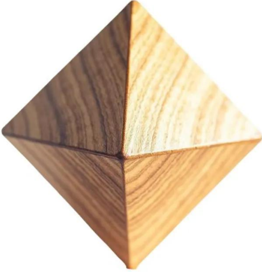
oktahendron
